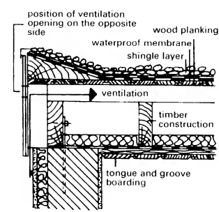
4 Cold roof in timber construction
